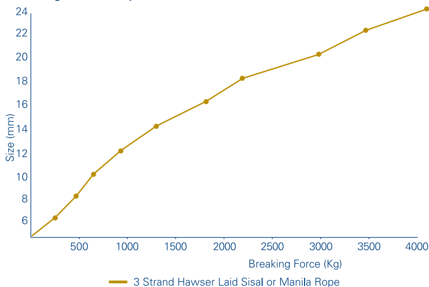
Breaking Force Graph
